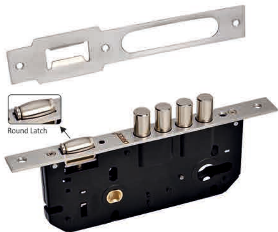
Lock Body 111
